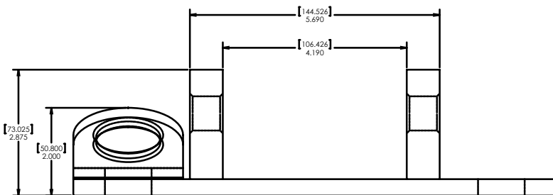
MODEL FB-SB3 FRONT VIEW
